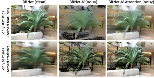
Figure 6. Feature aggregation by the NAN attention module (Sec. 4.2.2) : A demonstration of the importance and quality of individual features vs. joint statistics (mean, variance) in the clean vs. noisy regime, with and without our attention module. The columns compare denoising performance of IBRNet on clean images [left] and IBRNet- N on noisy images without [middle] and with [right] our attention module. The rows compare the influence of the features statistics (mean, variance) [top] to that of the individual features [bottom]. Please see text (in Sec 4.2.2) for a detailed discussion and interpretation of these results.
