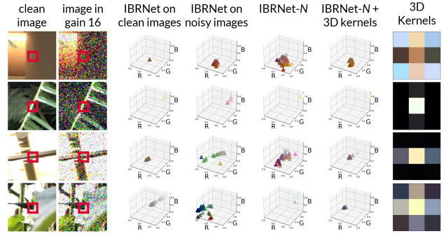
Figure 7. Influence of the NAN 3D-blending kernels (Sec. 4.3 and step III in Fig. 4) . [Left] Target pixels (clean and noisy with gain 16). [Center] Scatter plots in RGB-space of final predicted colors c_m along the ray through the pixel (we show only colors that are more influential in the final integration along the ray - the ones at locations with above-average density \rho_m ). These are shown for IBRNet on clean and noisy images, IBRNet- N on noisy images, and IBRNet- N with added 3D-blending kernels. [Right] The learned 3D-kernels associated with the ‘true’ pixel depth (we take the maximum-density sample), shown with RGB color-coding, scaled for clarity. See text for interpretation (Sec. 4.3).
